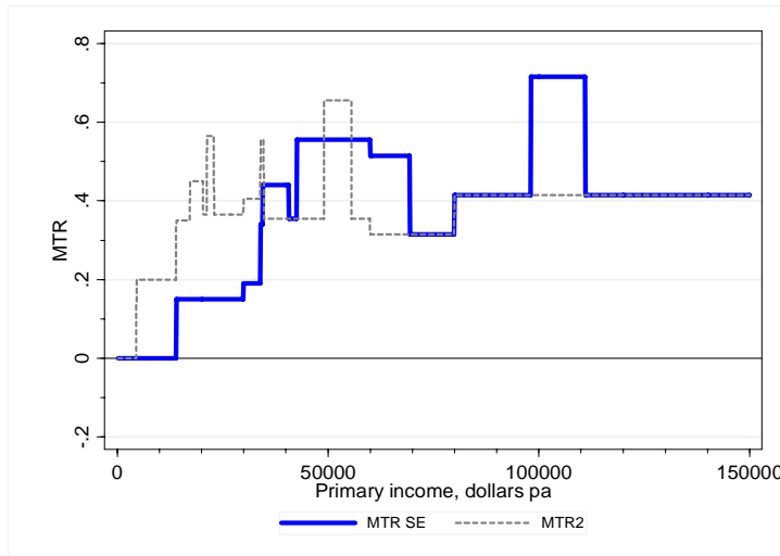
Figure 4.3a MTRs: PIT + LITO + FTBs + ML
